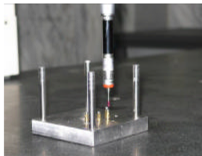
Fig. 9: Measuring over the ball top
