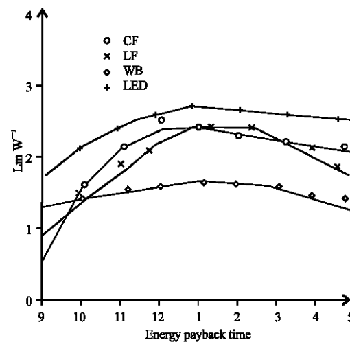
Fig. 2: Appliance lumen per watt over a period of time
