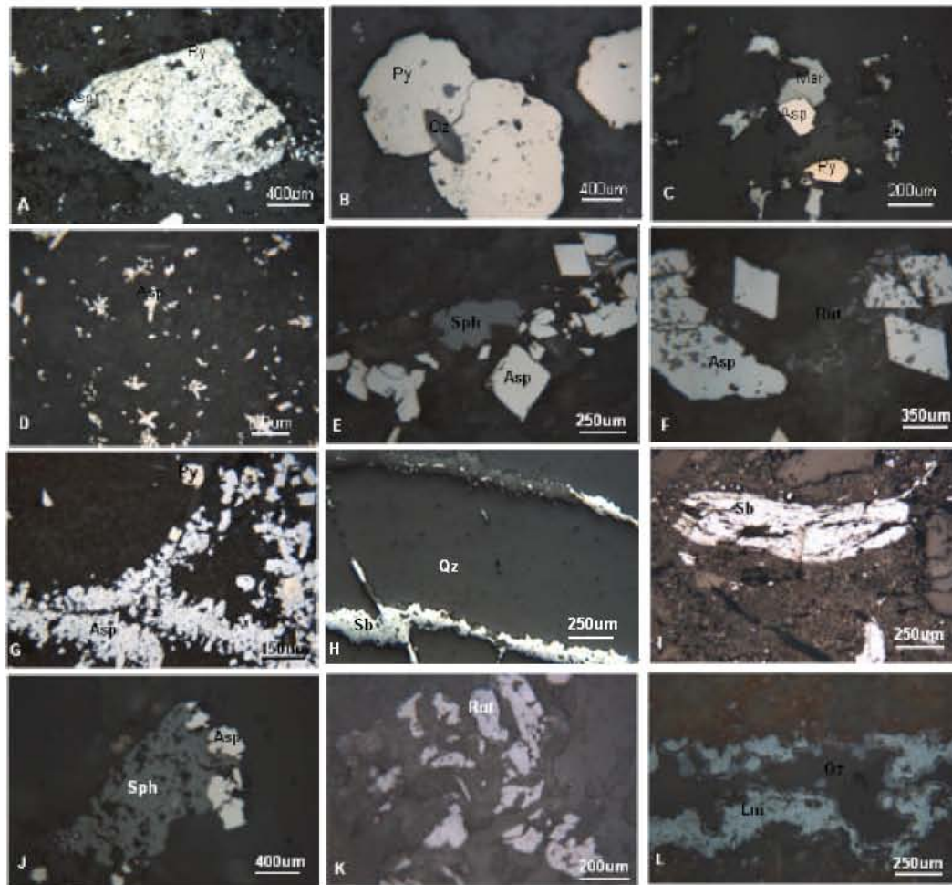
Fig. 3: Photomicrographs of ore fabric at Zaozigou Gold deposit polish sections (// / nicols. (A) A lens of pyrite in association with arsenopyrite. (B) Rounded pyrite with rim and later crystal of quartz automorph and inclusion of manganite (C) Association of pyrite, arsenopyrite and marcasite. (D) Disseminated star like arsenopyrite with pyrite. (E) Quartz veinlet fills with rhombic arsenopyrite, pyrite and sphalerite. (F) Rhombic arsenopyrite in gangue with inclusion of manganite and spot of manganite in the gangue. (G) Quartz veinlet with skeletal arsenopyrite and pyrite. (H) Quartz veinlet filling Stibnite. (I) Deformed Stibnite in quartz crystal as gangue. (J) Sphalerite replacing arsenopyrite. (K) Grain of Rutile in the altered zone. (L) Limonite forming along fracture filling silica
