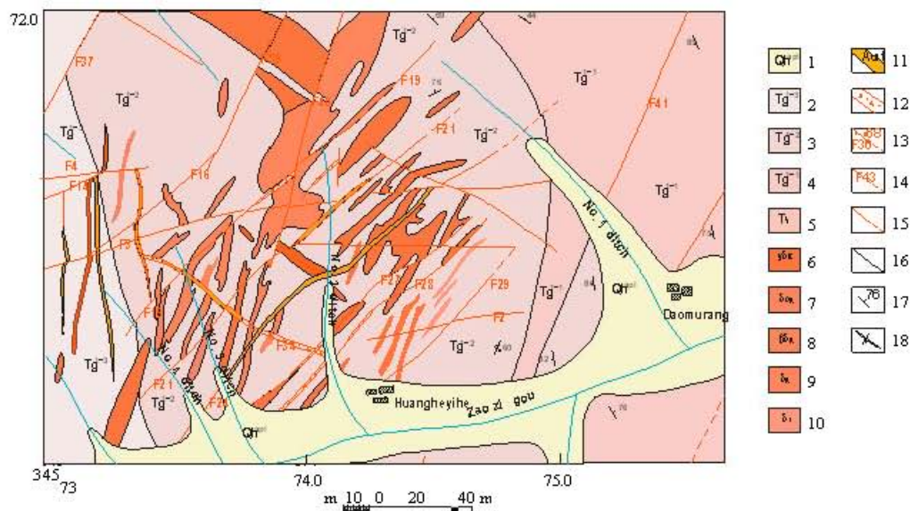
Fig. 2: Geological and structural map of Zaozigou: 1. Alluvial sand and gravel. 2. Grey calcareous slate with siltstone, arkose and oolitic limestone. 3. light-grey slate with quartz, sandstone limestone and gravel. 4. Dark grey siltstone slate, arkose limestone, sandstone. 5. Thick debris and fine arkose, fine slate. 6. Granodiorite porphyrite. 7. Quartz diorite porphyrite. 8. Biotite diorite porphyrite. 9. Diorite porphyrite. 10. Fine grained diorite 11 Orebodies. 12. Fault zone. 13. Reverse faults. 14. Speculated faults. 15. Geological boundaries. 16. Lithofacies boundaries. 17. Anticlinal axis. 18. Attitudes of stratum.
