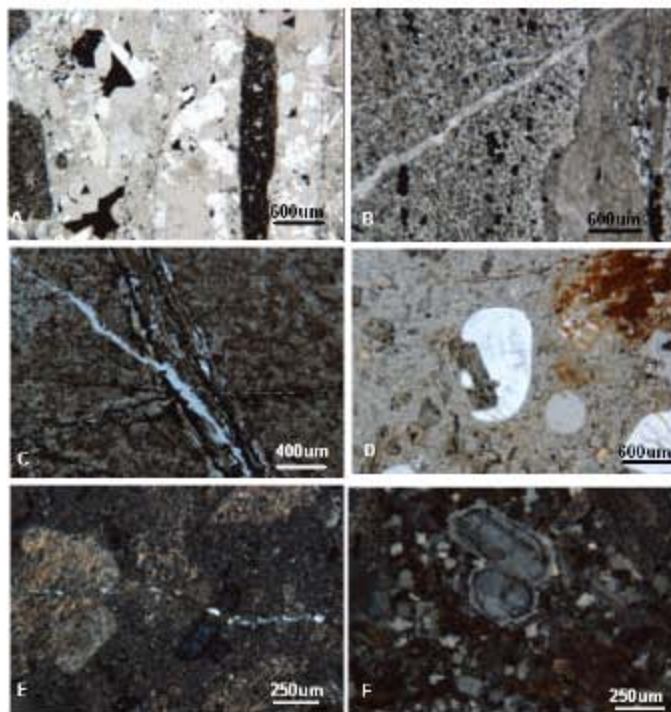
Fig. 4: Photomicrographs of thin section showing (A) Vugs and druse quartz (// nicols). (B) Sulfide minerals in the slate and calcite (// nicols). (C) Rounded crystal of quartz replaced by biotite (// nicols). (D) Anatomized quartz veinlet and Fe-oxide in the slate (// nicols). (E) Feldspar alteration into fine grains sericite, altered biotite crosscut by later quartz veinlet (x nicols). (F) Zoned feldspar, sericite and quartz crystals (x nicols).
