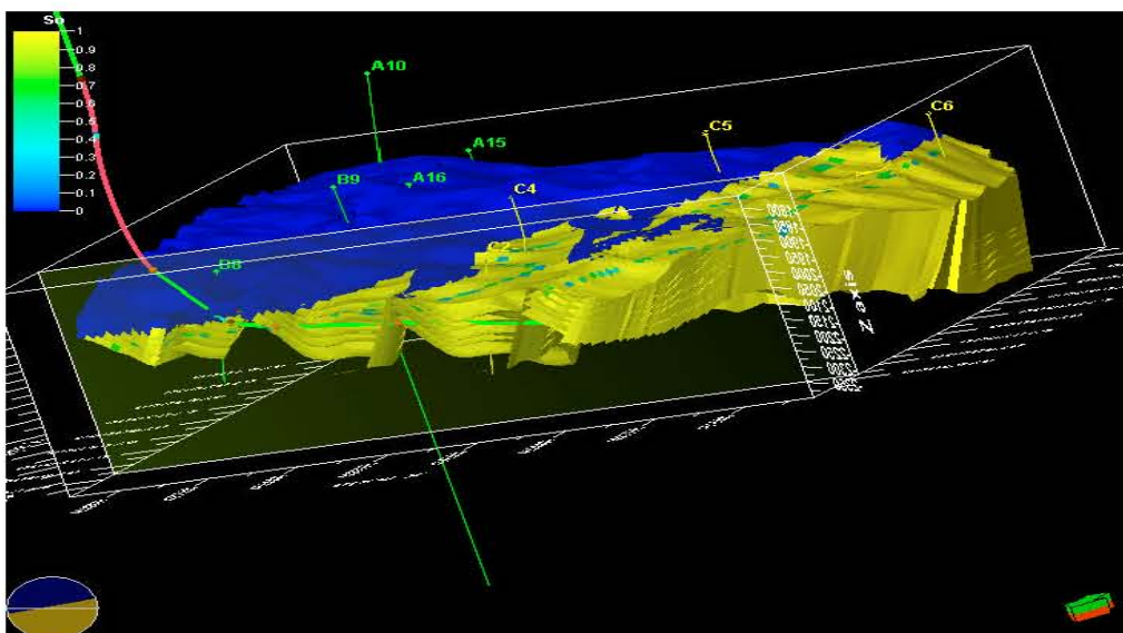
Fig. 6: Three-dimensional modeling of wells showing point of intersection with lithofacies in the reservoir
