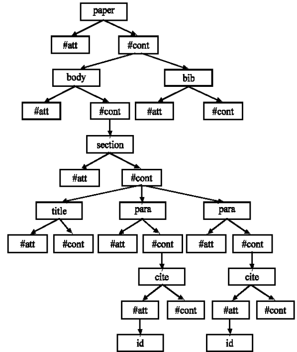
Fig. 4: The extended tree representation of an XML document in Fig. 2
