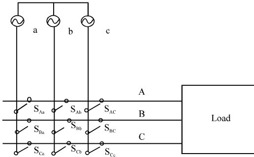
Fig. 4: Matrix converter
