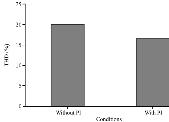
Fig. 15: Comparison of overall Voltage THD values under light load condition
