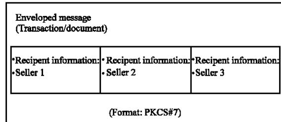
Fig. 6: The structure of a message with parallel envelopes
