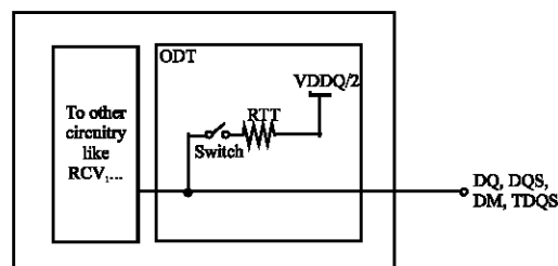
Fig. 8 : Functional representation of ODT
