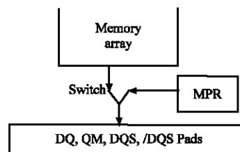
Fig. 4: Read leveling using MPR
