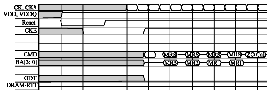
Fig. 2: Reset and initialization sequence
