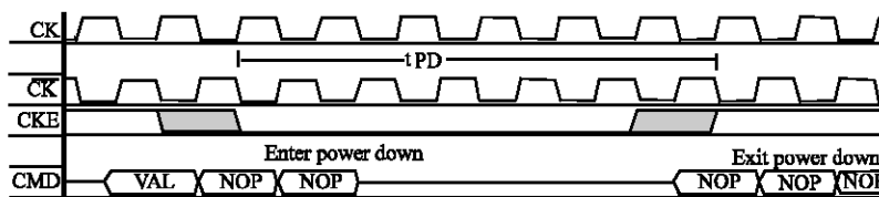
Fig. 7: Active power-down entry and exit timing diagram
