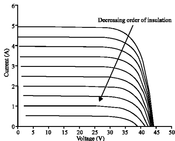
Fig. 1: I-V characteristics when insulation is changing
