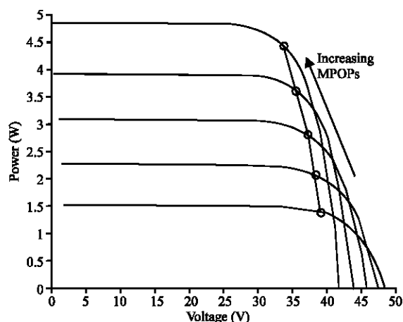
Fig. 9: MPOPs variation with insulation and temperature at the same time from P-V characteristics
