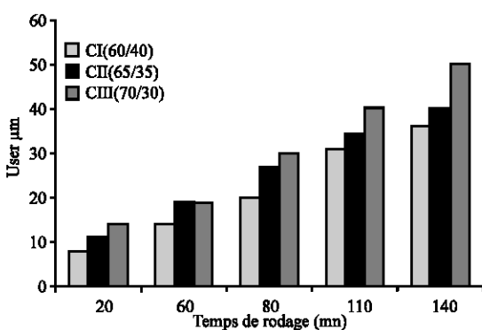
Fig. 4: Wear of the tool according to time
