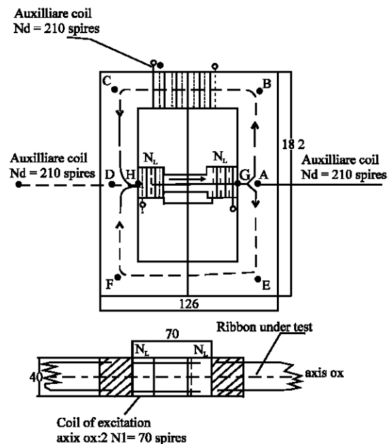
Fig. 2: Excitation circuit according to OX axis
