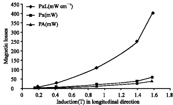
Fig. 9: Losses vs. induction in alternating field f=400\text{Hz}
