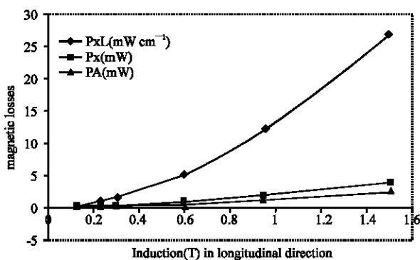
Fig 10: Losses vs. induction in alternating field characterisation f=50\text{Hz}
