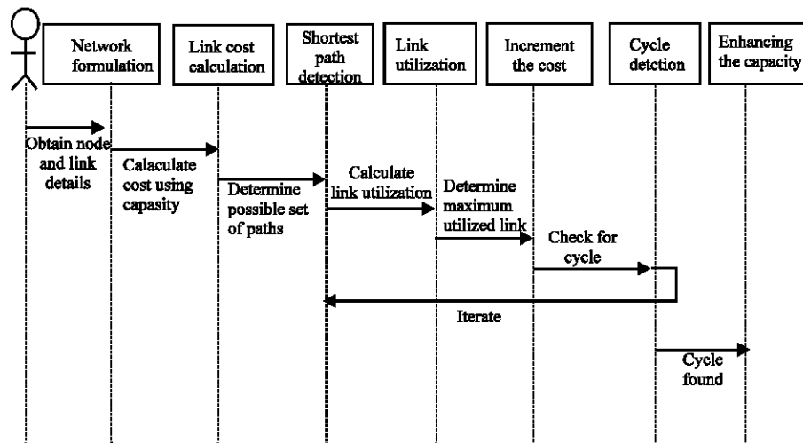
Fig. 5: Sequence diagram
