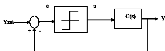
Fig. 2: Block diagram of relay feedback system
