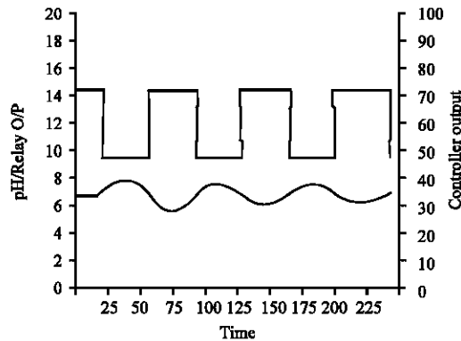
Fig. 6: RFB test for pH-middle
