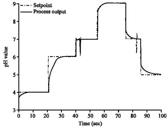
Fig. 10: Process response with set point change
