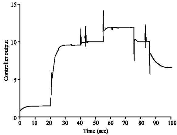
Fig. 11: Controller output
