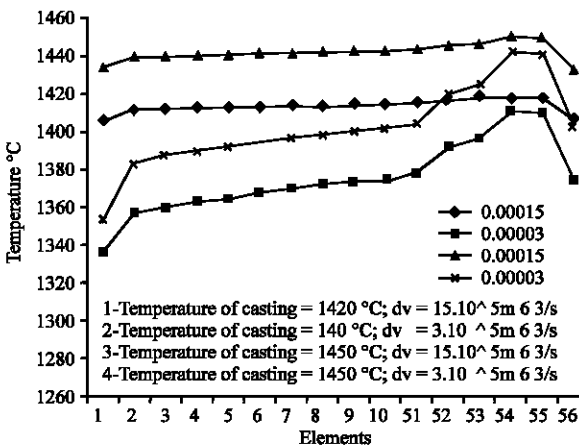
Fig. 5: Influence temperatures of the flow at speeds of filling
