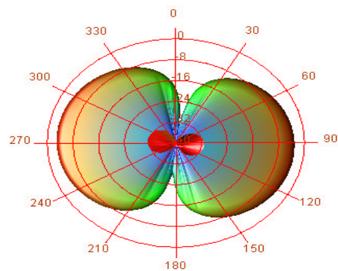
Fig. 3: Main lobe of the antenna simulated
