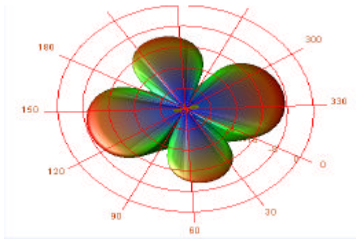
Fig. 4: Side lobes of the antenna simulated
