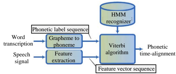
Fig. 3: HMM-based phonetic segmentation [18]
