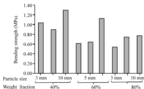
Fig. 9: Graphic of relation of pumice particle size and weight fraction upon bending strength (MPa)
