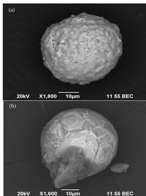
Fig. 2: a, b) Fe-O spherules photographed under a scanning electron microscope
