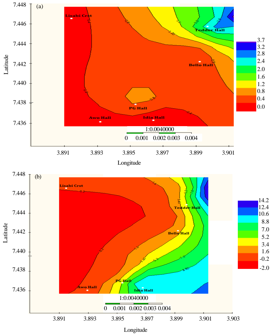
Fig. 7: a) Contour plots of the VES and b) pumping test derived t-values
