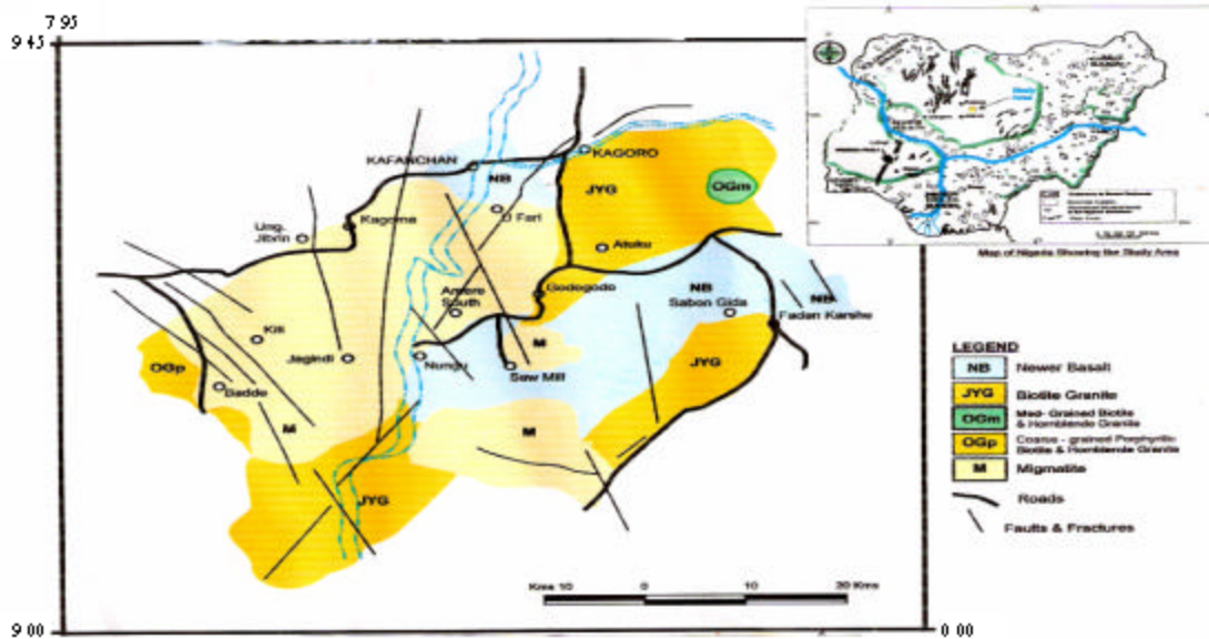
Fig. 2: Geological and structural map of the study area
