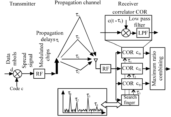
Fig. 2: RAKE receiver
