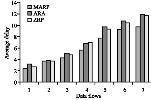
Fig. 7: Average delay with multimedia data flows
