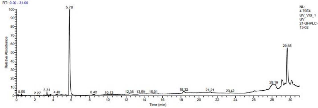
Fig. 7: Chromatogram peaks of bean ( Aquadulce ) by-products
