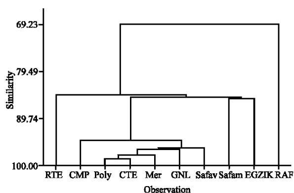
Fig. 2: Dendrogram with single linkage and squared pearson distance
