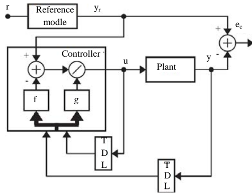
Fig. 2: NARMA-L2 controller
