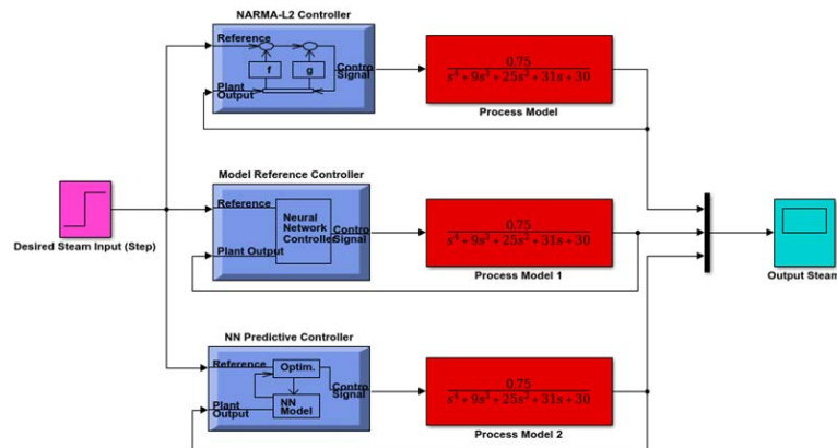
Fig. 5: Simulink model of the process control system with the proposed controllers for tracking the desired steam input step signal
