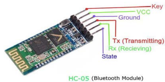
Fig. 3: Diagram of Bluetooth module HC05
