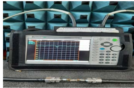
Fig. 3: Measuring the transmission co-efficient by using vector network analyser
