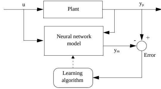
Fig. 4: Plant identification
