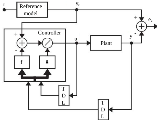
Fig. 2: NARMA-L2 controller
