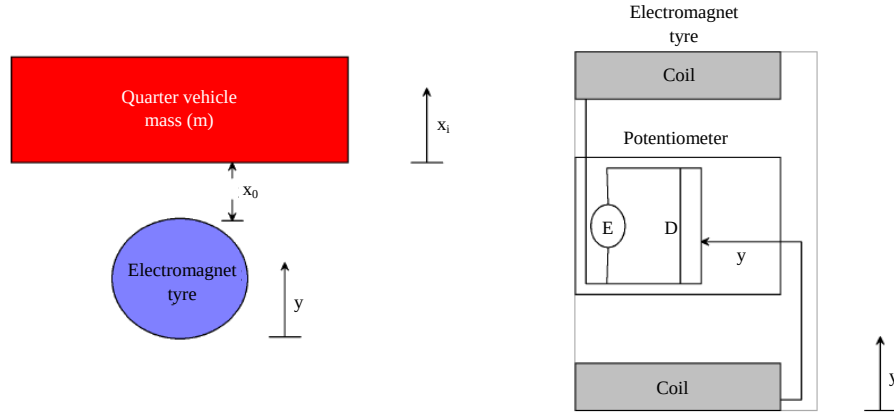
Fig. 1: Quarter vehicle electromagnetic suspension system and the electromagnetic tire design
