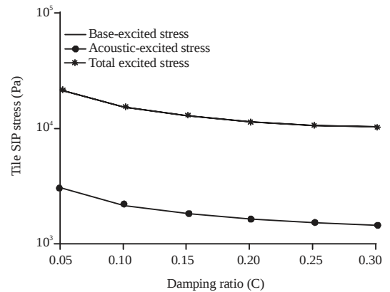
Fig. 27: Predication of three-sigma base, acoustic and total excited Stresses in tile/SIP of tile No. 6
