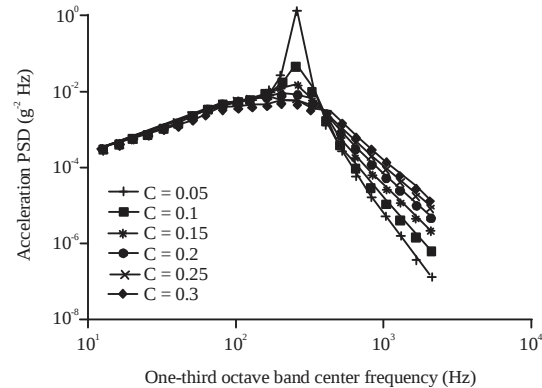
Fig. 11: Acceleration response of tile No. 2 of base-excited system
