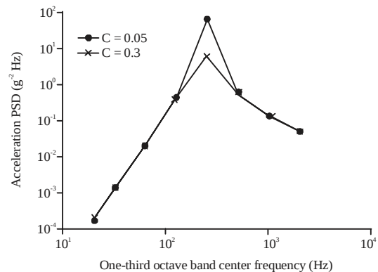
Fig. 19: Acceleration response of tile No. 4 of acoustic-excited system
