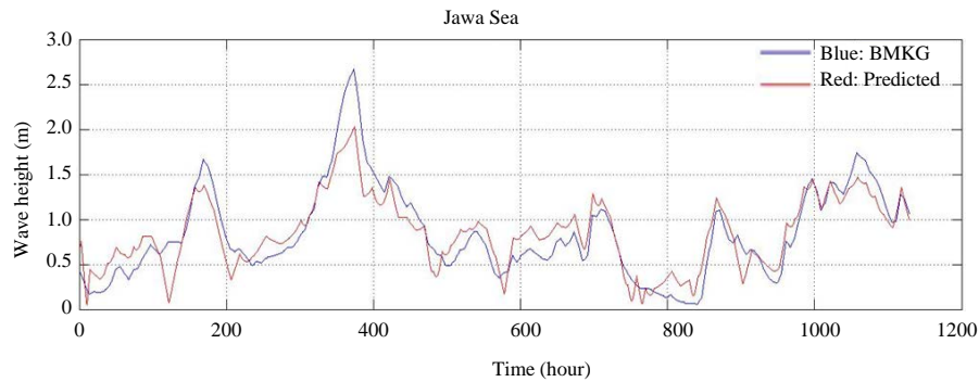
Fig. 4: Predicted Point B using Neural Network
