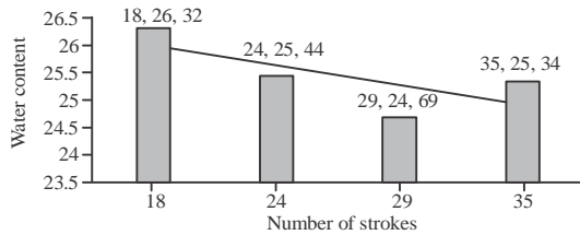
Fig. 10: Determination of plasticity index
