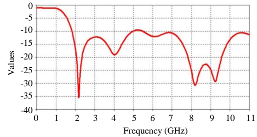
Fig. 5: The reflection coefficient of the prototype
