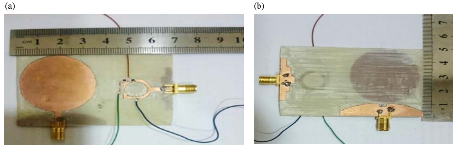
Fig. 12(a, b): Prototype of the fabricated interweave cognitive radio structure, (a) Front view and (b) Back view
