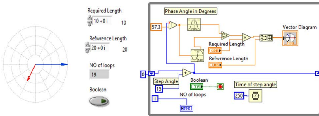
Fig. 10: Representation of single phase rotating phasor VI
