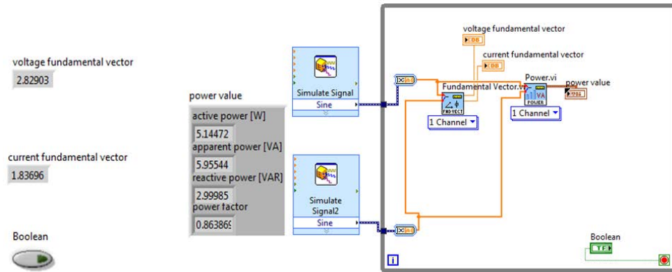
Fig. 1: Electrical power calculation using power VI
