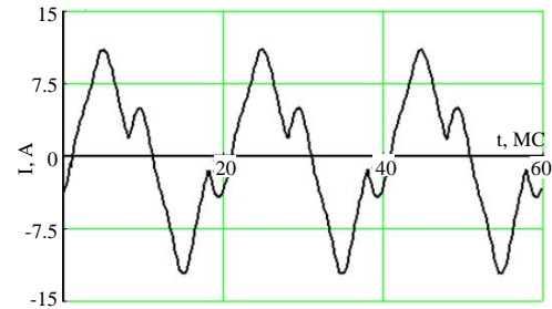
Fig. 7: Oscillogram of instantaneous values of current consumed by microwave oven
