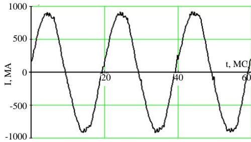
Fig. 4: Oscillogram of instantaneous values of the current of ELs with a rated power of 150 W, intended for street lighting in the grid power of 220V AC
