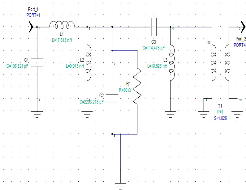
Fig. 6: Global schematic of the system
