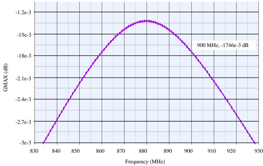
Fig. 8: Maximum gain measurement
