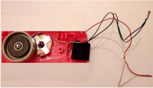
Fig. 4: Generator-emitter fabrication
