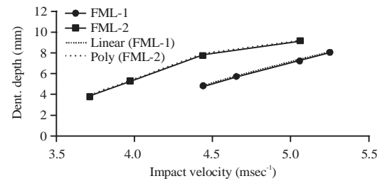
Fig. 7: FMLs, indentation depth versus the impact velocity
