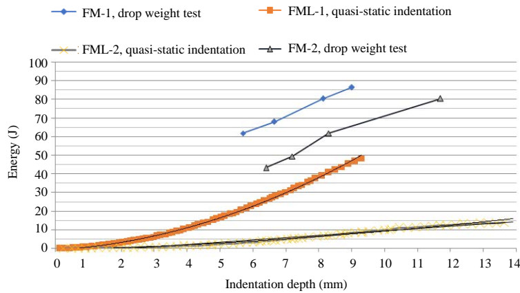
Fig. 10: FMLs, comparison between the quasi-static indentation test and drop weight impact test
