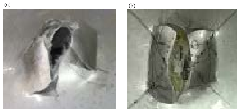
Fig. 4(a, b): FMLs, specimen after quasi-static test, (a) FML-1 and (b) FML-2
