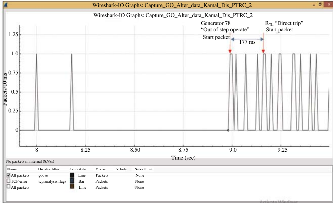
Fig. 20: Initiating and triggered GOOSE packets
