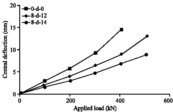
Fig. 11: Central deflection-applied load relationship for group 2 slabs ( f_c' = 34.7 MPa)
