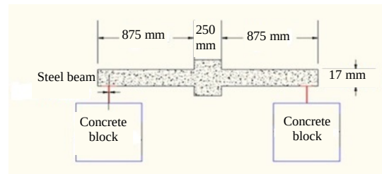
Fig. 5: Experimental set-up of slabs showing the dimensions
