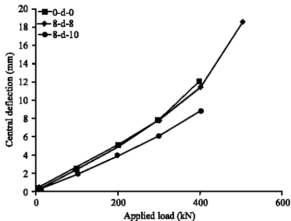
Fig. 10: Central deflection applied load relationship for group 1 slabs ( f_c' = 40.7 MPa)
