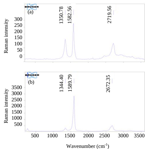
Fig. 5: Raman spectra for: a) MWCNTs and b) SWCNTs
