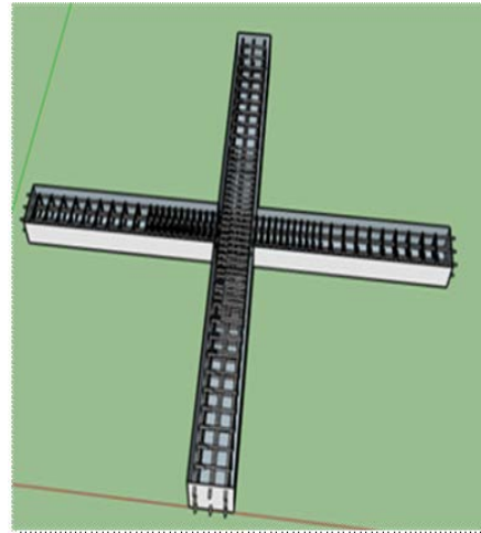
Fig. 4: Monolith joint (BN)
