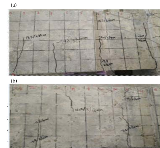
Fig. 15a, b): The cracks on plastic hinge area (BTK 30)
