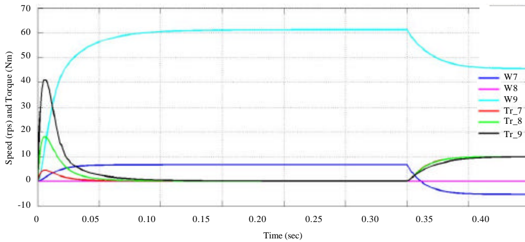
Fig. 15: Rotor speed and electromagnetic torque at 10 Nm load
