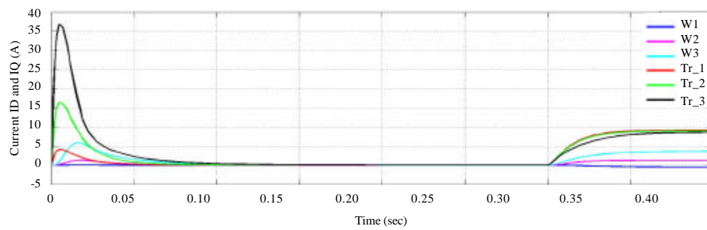
Fig. 12: Coordinate system current d-q axis at varying voltage at 10 Nm load
