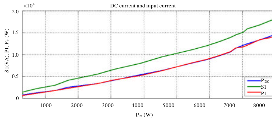
Fig. 21: Relation between PDC (W), input power (W), active power (VA) with shift power (W)
