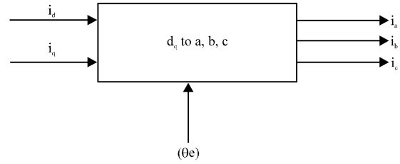
Fig. 3: i_d-i_q to i_a, i_b, i_c transformation block
