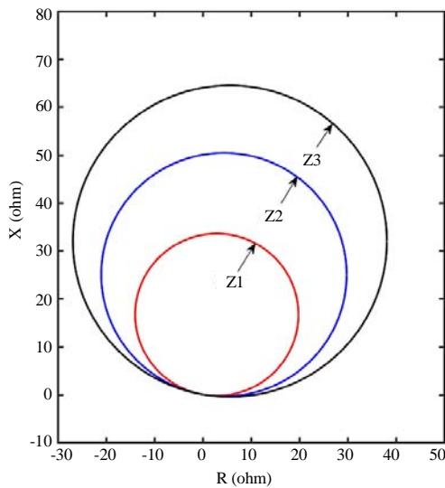
Fig. 7: Impedance characteristics of R_{TL}
