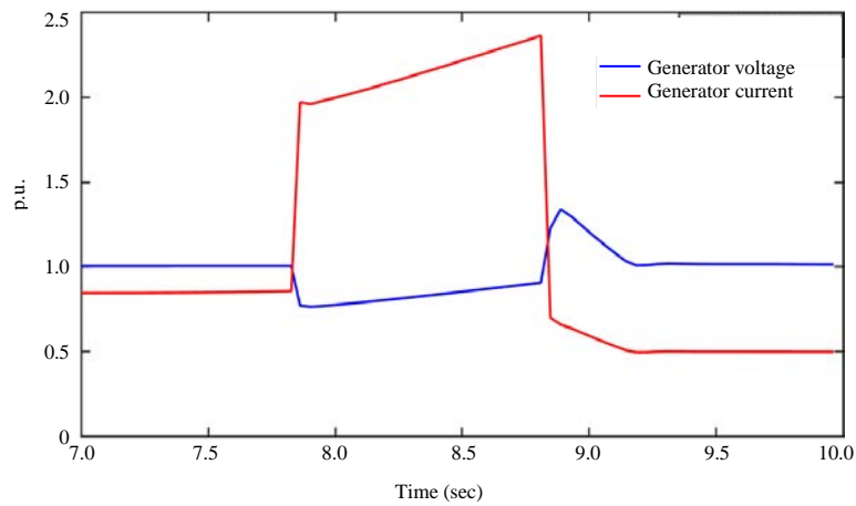
Fig. 10: Generator current and terminal voltage during and after the fault conditions
