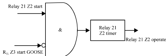
Fig. 12: Logic implemented in the generator protection relay
