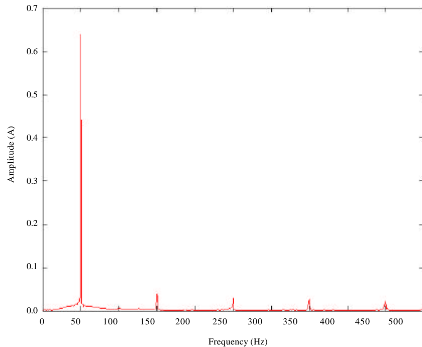
Fig. 6: The signal of power source from PLN with charging cellphone as load (Hormonic spectrum)
