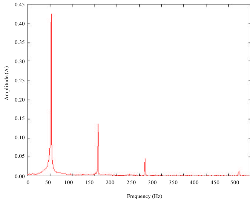
Fig. 5: The signal of power source from microgrid with light bulb as load (Hormonic spectrum)
