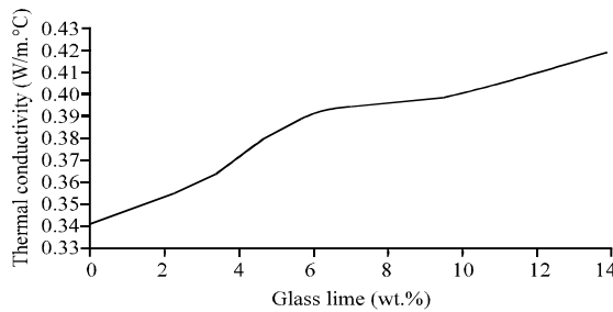
Fig. 2: The relationship between thermal conductivity and wt.% glass lime
