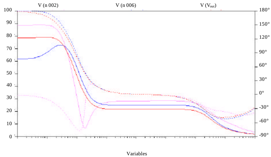
Fig. 12: Effect of R8 open on each stage
