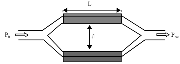
Fig. 2: Mach-Zehnder Interferometer (MZI) based optical switch
