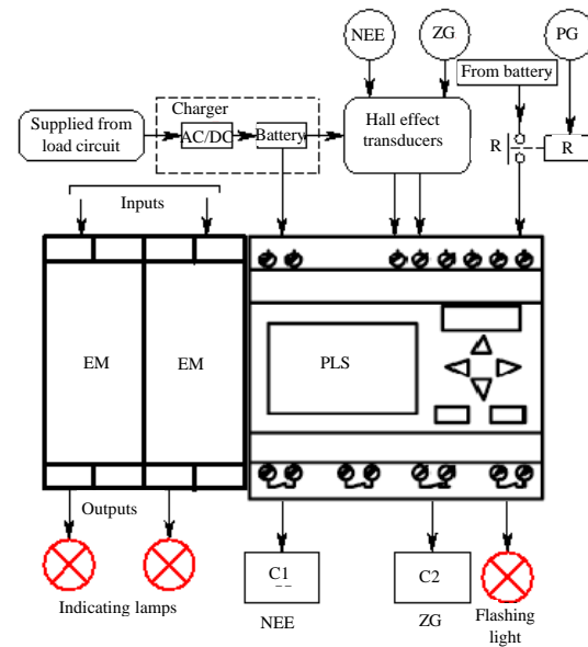
Fig. 3: External connections of the control circuit of ATS
