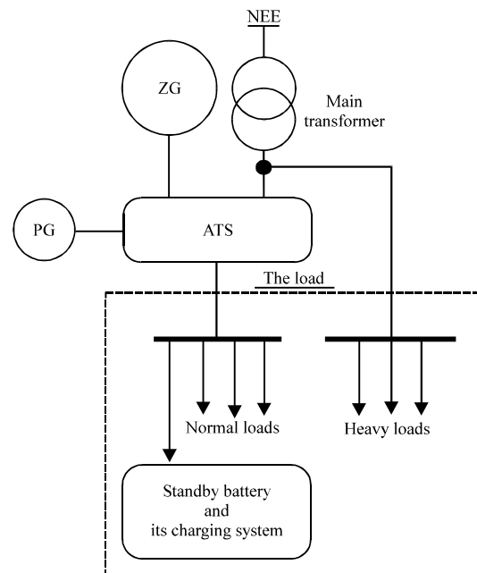
Fig. 1: General electrical power scheme
