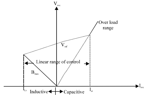
Fig. 2: V-I characteristics of SVC
