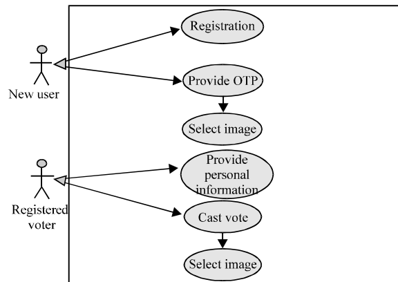
Fig. 4: Use case diagram of the system
