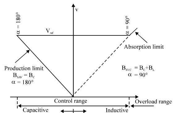
Fig. 7: Operating characteristics of FC-TCR
